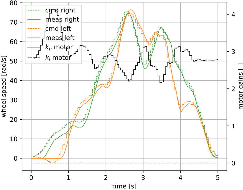
Wheel Speeds
